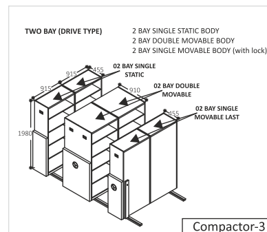
Drive Type Compactor COMPACTOR-3
